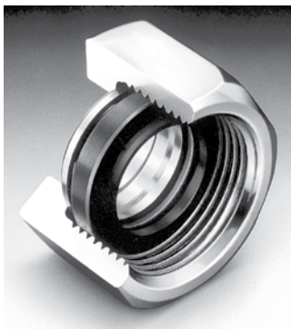
Fig. E5 — The unique Functional Nut allows easy handling and quick assembly.
