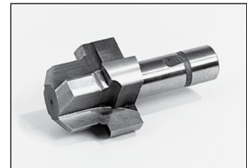
Fig. R83 — SAE Straight Thread Port Counterboring Tool
