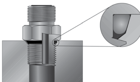
Fig. S7 — Non-Adjustable Port End Assembly
