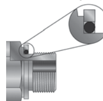
Fig. F5 — O-Ring with Retaining Ring
