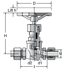
Flow Direction Internal threaded spindle and body of low grade forged stainless steel
