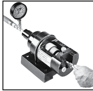
Fig. S27 – Flaring with Hydra-Tool
